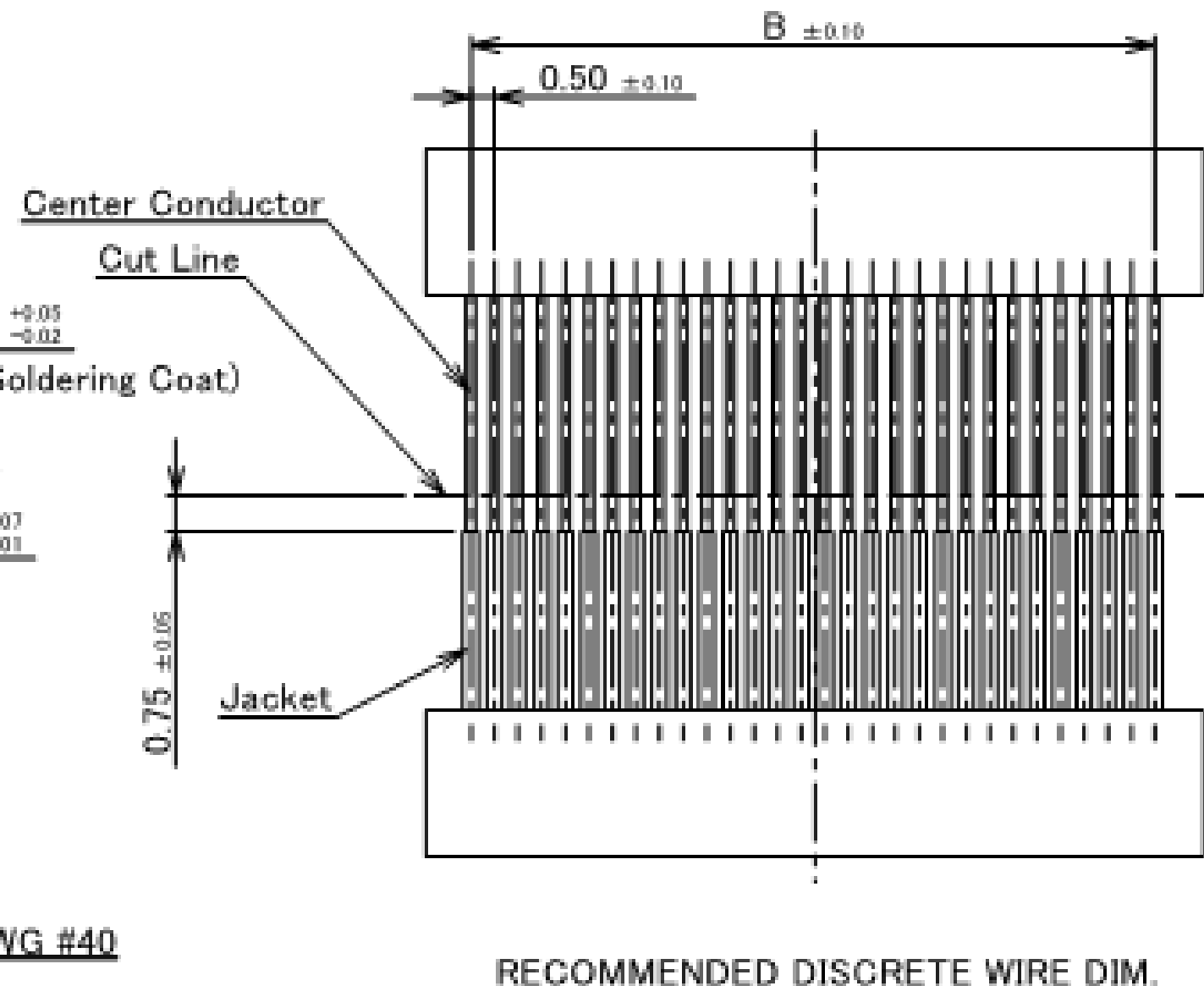
RECOMMENDED DISCRETE WIRE DIM.
